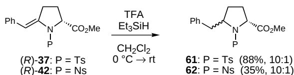
Scheme 10.
