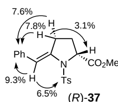
Figure 1. 1 H NMR NOE data of enamide (R)-37.
