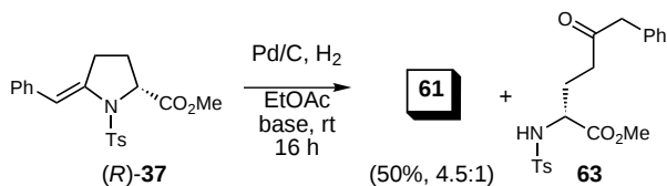
Scheme 11.
