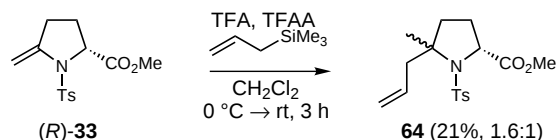
Scheme 12.
