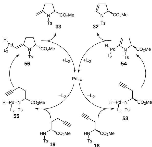
Scheme 7.
