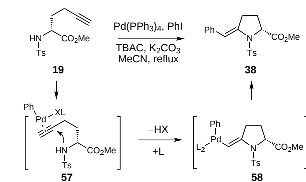
Scheme 8.
